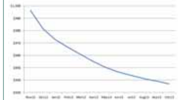
Gasoil forward price in US$ per tonne
